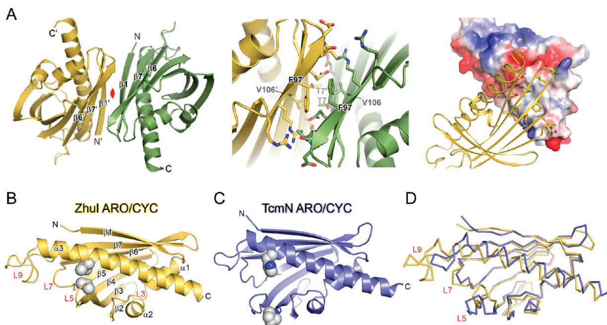
Figure 4. Overall structure of ZhuI and a comparison with TcmN ARO/CYC. (A) ZhuI dimer structure (left). \beta -Strands at the dimer interface are labeled, and the noncrystallographic 2-fold rotation axis relating the two monomers is colored red. Close-up view of the dimer interface (middle). Illustration of the complementarity and chemical nature of the dimer contact surface (right). One monomer is represented as an electrostatic surface (red for electronegative, blue for electropositive, and gray for neutral), and the other is drawn as a cartoon with interacting residues as sticks. (B) Monomer structure of ZhuI with secondary structure elements labeled and two interacting residues (V55 and V138) shown as spheres. (C) Crystal structure of TcmN ARO/CYC with residues P56 and H128 (structurally equivalent to those listed for panel B) drawn as spheres (see the sequence alignment in Figure 3B). (D) Backbone overlay of ZhuI and TcmN ARO/CYC.
