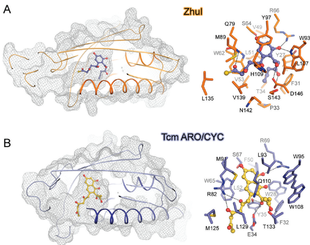
Figure 6. Docking of putative polyketide intermediates into the ARO/CYC pocket. (A) Docking of the 18-carbon intermediate 1 (Figure 1), the putative product of ZhuI. (B) Docking of a putative 20-carbon bicyclic aromatic intermediate with TcmN ARO/CYC. For both panels, the left image is a cutaway mesh surface view showing the positions of the docked molecules and the right image is a view of interactions of pocket residues with the docked compounds.
