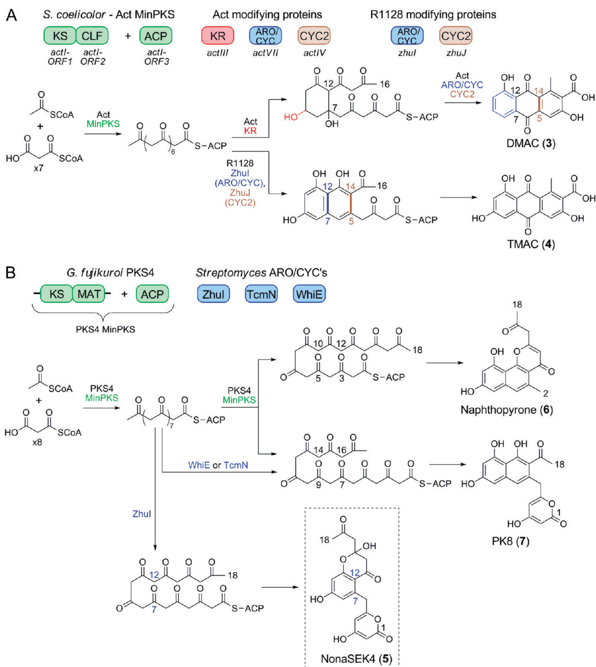
Figure 2. Influence of ZhuI on first-ring cyclization specificity in engineered biosynthesis. (A) Combination of the Act MinPKS, KR, ARO/CYC, and CYC proteins from S. coelicolor results in production of the octaketide DMAC. In comparison, when ZhuI and ZhuJ are combined with the Act MinPKS, they direct C7–C12 and C5–C14 cyclization of an unreduced octaketide chain to yield TMAC (4). (B) In vitro reconstitution of polyketide biosynthesis using the PKS4 minPKS from Gibberella fujikuroi results in the production of naphthopyrone 6 and PK8 (7). The addition of C9–C14 cyclase TcmN or WhiE results in the exclusive production of 7. In contrast, the addition of ZhuI directs the regiospecific C7–C12 cyclization of the nonaketide chain to yield a novel polyketide, NonaSEK4 (5). Note that TcmN and WhiE direct two consecutive cyclizations (C9–C14 and C7–C16), whereas ZhuI promotes only a single cyclization event between C7 and C12.
