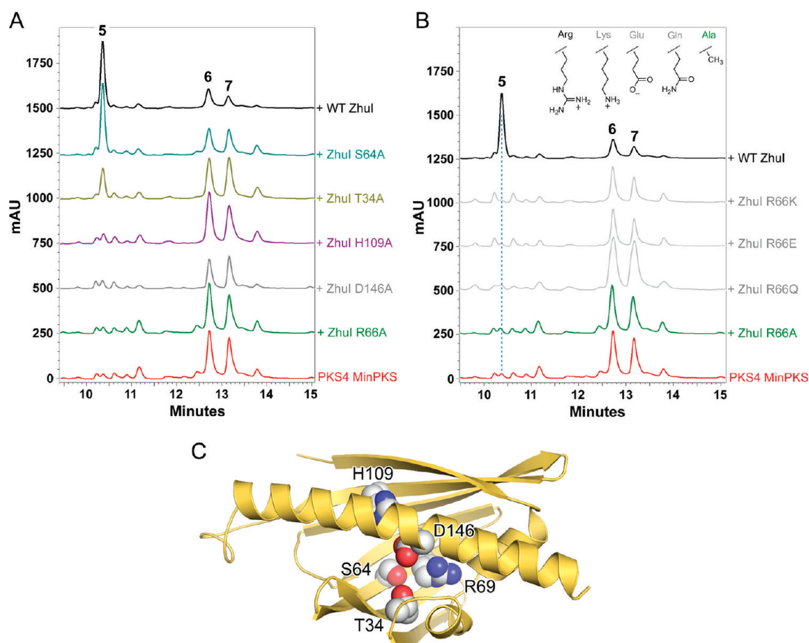
Figure 7. Results of ZhuI pocket residue mutagenesis as tested in vitro. (A) HPLC analysis (traces displayed at 270 nm) of the product profiles obtained by in vitro reconstitution of polyketide biosynthesis utilizing the PKS4 minPKS with WT or mutant ZhuI ARO/CYC. (B) Product profiles of additional pocket arginine mutants (R66Q, R66E, and R66K). The inset shows the amino acid side chain groups at residue position 66 for WT and mutant ZhuI as assayed. (C) Structure of ZhuI showing the mutated pocket residues as spheres.
