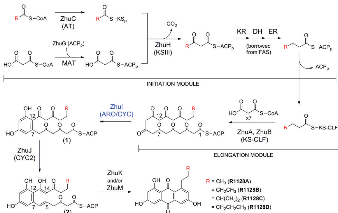
Figure 1. Proposed biosynthetic pathway of the zhu PKS from Streptomyces sp. R1128.
