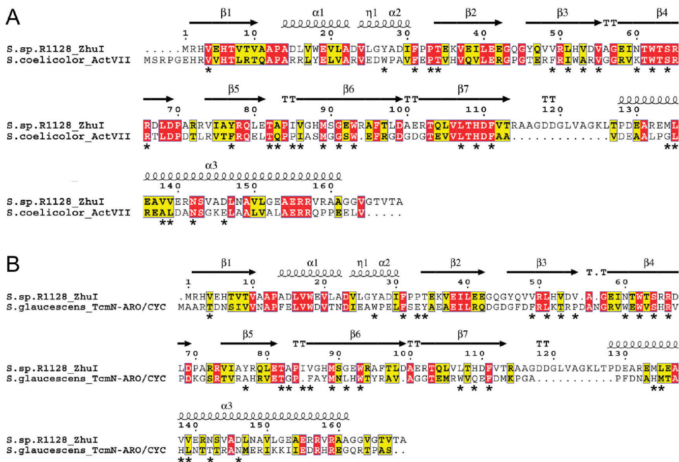
Figure 3. Sequence alignment of ZhuI ARO/CYC with (A) the N-half ARO/CYC domain (residues 1–156) of the didomain protein ActVII from S. coelicolor and (B) the ARO/CYC domain (residues 1–157) of TcmN from Streptomyces glaucescens . ActVII is associated with dehydration and aromatization of a C7–C12 cyclized first ring, whereas TcmN ARO/CYC is associated with C9–C14 first-ring cyclization. Secondary structure elements shown on the top of each alignment are identified according to the ZhuI structure, and asterisks below the alignments denote pocket-defining residues.
