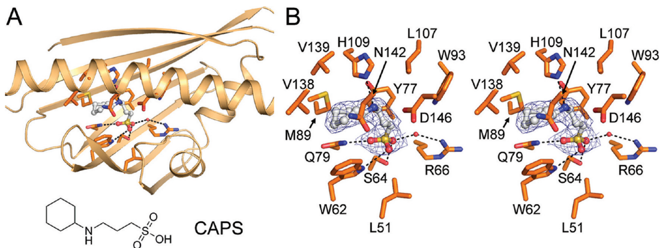
Figure 5. Structure of ZhuI with CAPS bound. (A) Overall view with the protein backbone rendered as a cartoon and residues within 4 Å of the CAPS molecule drawn as sticks. Potential hydrogen bonds are represented as dashed lines. The structure of CAPS ( N -cyclohexyl-3-aminopropanesulfonic acid) is drawn below ZhuI. (B) Stereoview of interacting residues. Blue mesh around the bound ligand is derived from the 2.4 \text{ \AA } |2F_o - F_c| electron density map contoured to 0.8\sigma .
